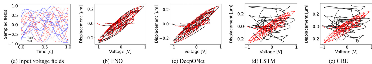
FIG. 5. Performance of neural network models in predicting hysteresis loops described by (4) for Gaussian random fields. Input voltage fields used for training and testing (a) followed by performance of various methods (b)–(e). The solid black curve denotes the predictions, and the dashed red line depicts the ground truth.
