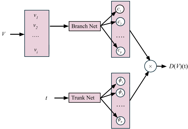
FIG. 2. Deep Operator Network (DeepONet) architecture comprising two independent feedforward neural networks—the branch net and the trunk net—whose outputs are combined through a dot product to approximate the displacement.
