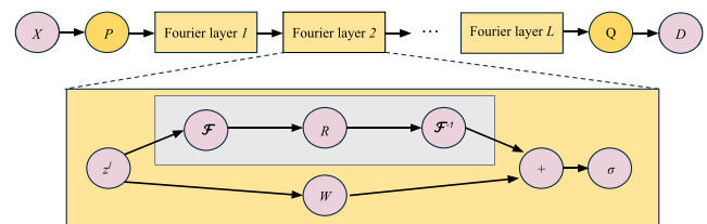
FIG. 1. Neural architecture for Fourier neural operator (FNO). The input X := [v, t] is passed through projection tensor ( P ) and Fourier layers and finally downsampled ( Q ) to approximate the displacement.
