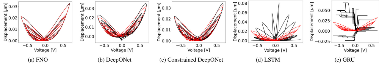
FIG. 4. Performance of neural network models in predicting hysteresis loops described by (8) for sinusoidal voltage fields. The solid black curve denotes the predictions, and the dashed red line depicts the ground truth.
