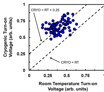
Fig 8: Cross wafer distribution of cryogenic V_T ( T \sim 1.9 K) vs Room Temperature V_T across a full 300mm wafer. The data show correlation with a systematic increase in V_T at low temperature.
