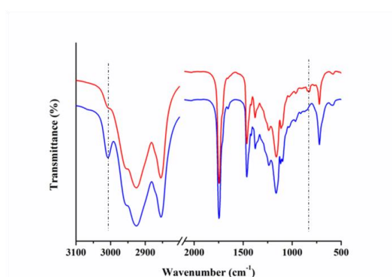
Figure 4. FT-IR spectra of glyceryl trioleate before (blue) and after the epoxidation (red). The characteristic peaks of the C=C-double bond ( 3007\text{ cm}^{-1} ) and for the oxirane ring ( 831\text{ cm}^{-1} ) are highlighted.
