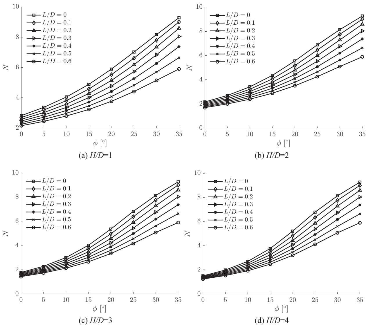
Fig. 9. Variations of N with \phi for various L/D under (a) H/D = 1 ; (b) H/D = 2 ; (c) H/D = 3 ; (d) H/D = 4 .
