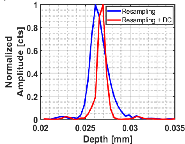
Figure 3: Axial point spread function measured using a mirror placed at a depth (in air) of 25 \mu\text{m} .
