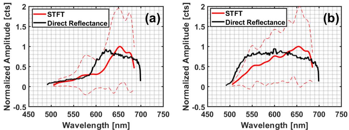
Figure 6: Measured spectral reflectance using the Vis-OCT system. (a) Red paint layer, (b) Yellow paint layer. Average values (continuous lines), standard deviation (dashed lines).
