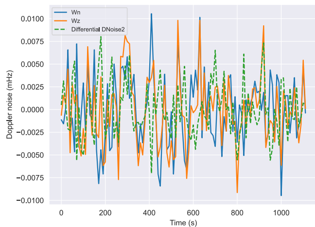
Figure 9. The Doppler noise (DNoise2) comparison between Wz and Wn from the session held on 6 August 2015. The spacecraft is further away from the Sun with a solar elongation of 15.31 degrees; hence, we start to see significant contributions from instrumental noises and not the solar plasma propagation dominating. Thus, we don't see the same strong correlation as the previous session.
