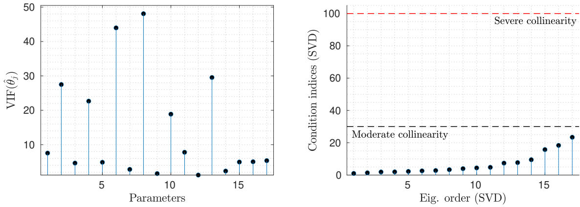
Fig. 6 Variance Inflation Factors and SVD condition indices of the spline model for C_m
