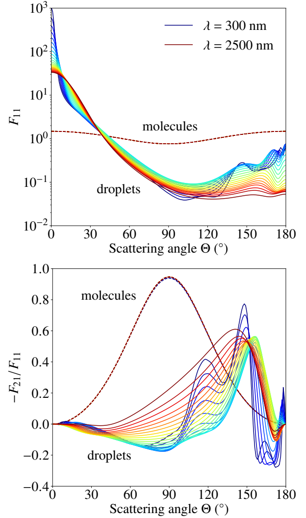
Fig. 5. Phase function F_{11} (element (1,1) of scattering matrix \mathbf{F}_{\text{sca}} ) (top) and degree of linear polarization ( -F_{21}/F_{11} ) (bottom) as functions of the scattering angle \Theta , for singly scattered light by gaseous molecules (dashed lines) and cloud droplets (solid lines). Scattering angle \Theta is the angle between the directions of propagation of the incident and the scattered light ( \Theta = 180^\circ - \alpha ). The wavelengths range from 300 nm (dark blue line) to 2500 nm (dark red line), in steps of 100 nm. The lines for the gaseous molecules at the different wavelengths virtually overlap.
