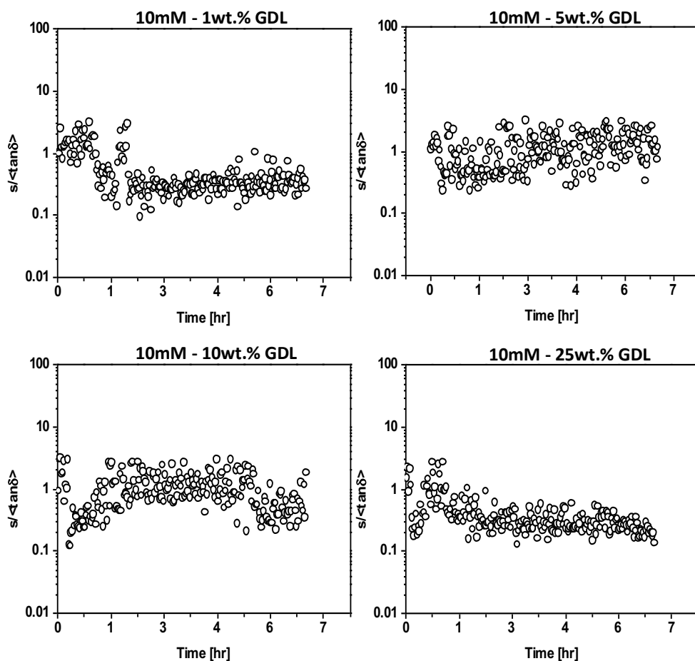
Figure S23. \tan\delta analysis for data obtained at a gelator concentration of 10mM and 1wt.% (57 mM), 5wt.% (295 mM), 10wt.% (624 mM), 25wt.% (1871 mM) of GDL. The corresponding [GDL]/[Gelator] molar ratios are 5.7, 29, 62 and 187 respectively.
