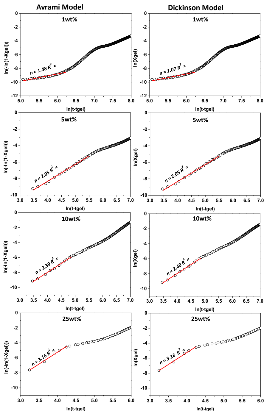
Figure S9. Model fits based on Avrami and Dickinson models for case of 10mM gelator concentration and 1wt.% (57 mM), 5wt.% (295 mM), 10wt.% (624 mM) and 25 wt.% (1871 mM) of GDL. The corresponding [GDL]/[Gelator] molar ratios are 5.7, 29, 62 and 187 respectively.
