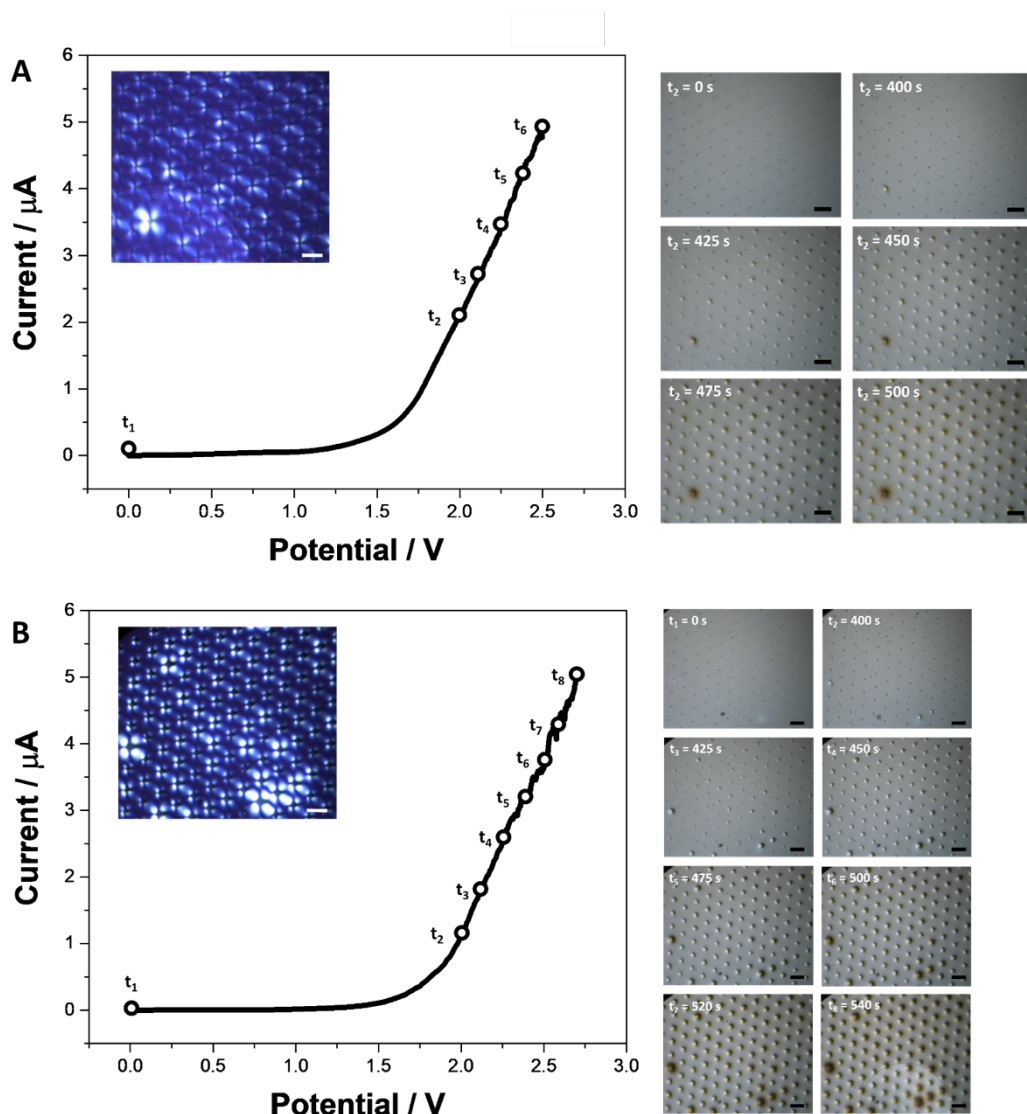
Figure S8. The linear sweep voltammograms recorded in the A – 15 mM and B – 25 mM \text{Na}_2\text{DBC} solution at 5 \text{ mVs}^{-1} . On the right from the voltammograms one can find the set of the corresponding optical microscopy images recorded at different deposition times (marked on the upper left corner). The inset of each linear sweep voltammogram is the polarization microscopy image recorded after hydrogel deposition. The scale bars correspond to 50 \mu\text{m} each.
