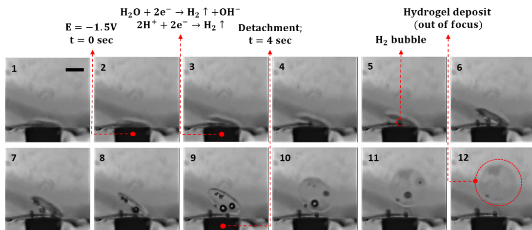
Figure 6. Images from 1 to 12 are the frames taken from the movie recorded during electrochemically controlled detachment of a hydrogel deposits formed at E = 1.5\text{ V} in 40\text{ mM Na}_2\text{DBC} in 500\text{ mM NaNO}_3 for 150 seconds (see image 1 for the corresponding deposit). The images are saturated with grey colour in order to increase the contrast. Scale bar – 100\text{ }\mu\text{m} .
