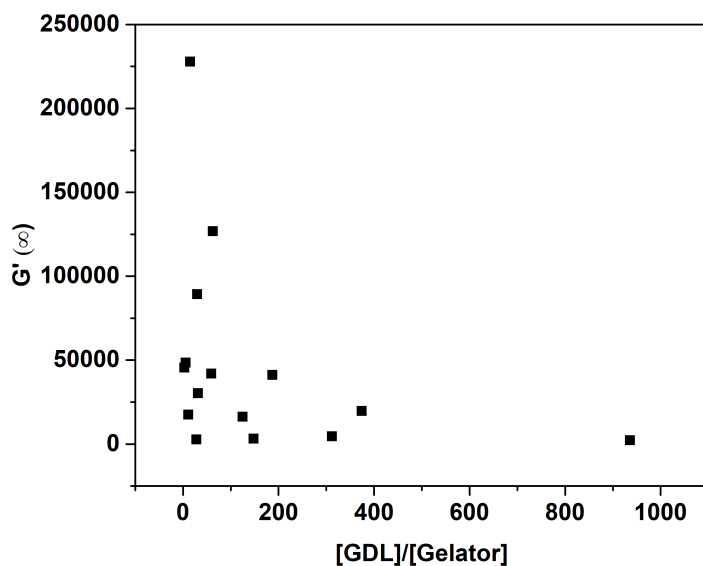
Figure S28. Plot of plateau modulus ( G'(\infty) ) at various [GDL]/[Gelator] molar ratios (GDL - 1wt.% (57 mM), 5wt.% (295 mM), 10wt.% (624 mM), 25wt.% (1871 mM), 25wt.% (1871.2 mM), Gelator – 2mM, 5mM, 10mM, 20mM)
