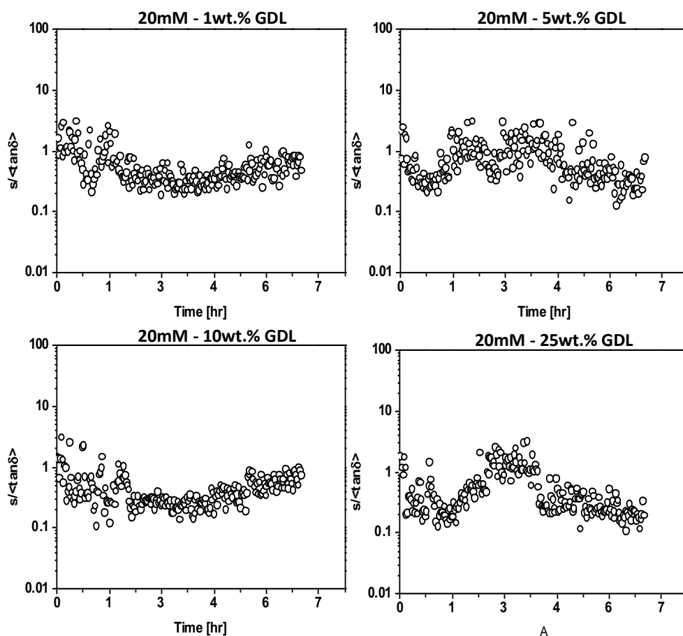
Figure S24. Tan \delta analysis for data obtained at a gelator concentration of 20mM and 1wt.% (57 mM), 5wt.% (295 mM), 10wt.% (624 mM), 25wt.% (1871 mM) of GDL. The corresponding [GDL]/[Gelator] molar ratios are 2.8, 15, 31 and 93 respectively.
