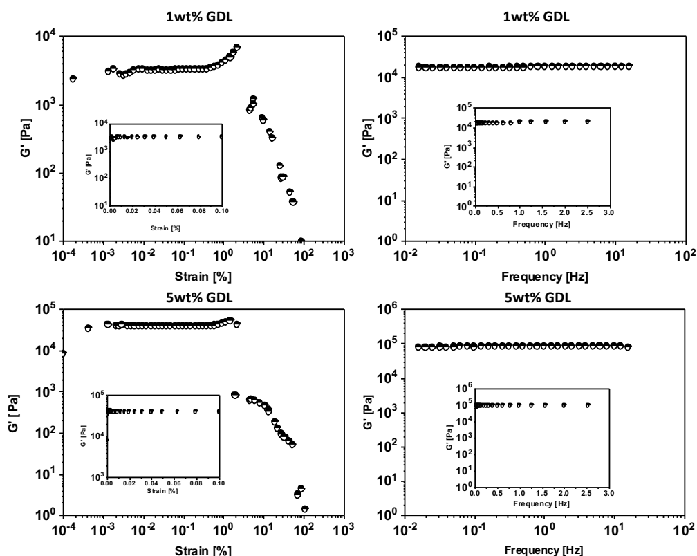
Figure S17. Strain and frequency sweeps at gelator concentration = 5mM and 1wt.% (57 mM) and 5wt.% (295 mM) of GDL. The corresponding [GDL]/[Gelator] molar ratios are 11 and 59 respectively.
