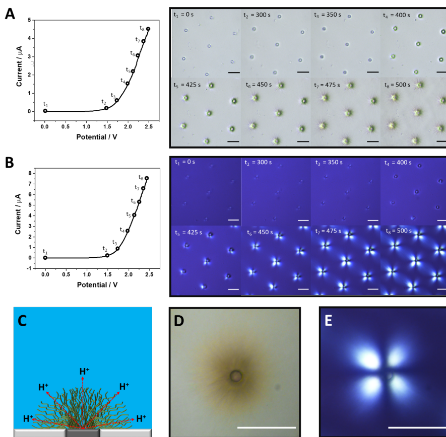
Figure 4. A and B represent linear sweep voltammograms recorded in 10 mM \text{Na}_2\text{DBC} and 500 mM \text{NaNO}_3 solution at 5 \text{ mV}\cdot\text{s}^{-1} with corresponding sequence of optical microscope images (on the right from voltammograms) recorded during voltametric hydrogel deposition (A – normal microscopy; B – polarization microscopy)). C is the schematic representation (to the best of our understanding) of the hydrogel deposit grown over platinum microelectrode. D and E are the images taken at higher magnification under optical and polarization microscopy respectively after deposition process. The single electrode DIA = 10 \mu\text{m} ; S (pore centre to centre distance) = 100 \mu\text{m} . The scale bars are equal to A and B – 100 \mu\text{m} and D and E – 50 \mu\text{m} .
