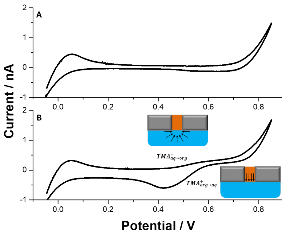
Figure S3. Ion transfer voltammograms recorded at the micro-pore supported interface between 10 mM NaCl and 10 mM BTPPA + TPBCl - in the absence (A) and in the presence (B) of 40 μM TMA + Cl - . The current of the forward wave (0.25 nA) correspond to pore radii equal to 12 μm (24 μm in diameter).
