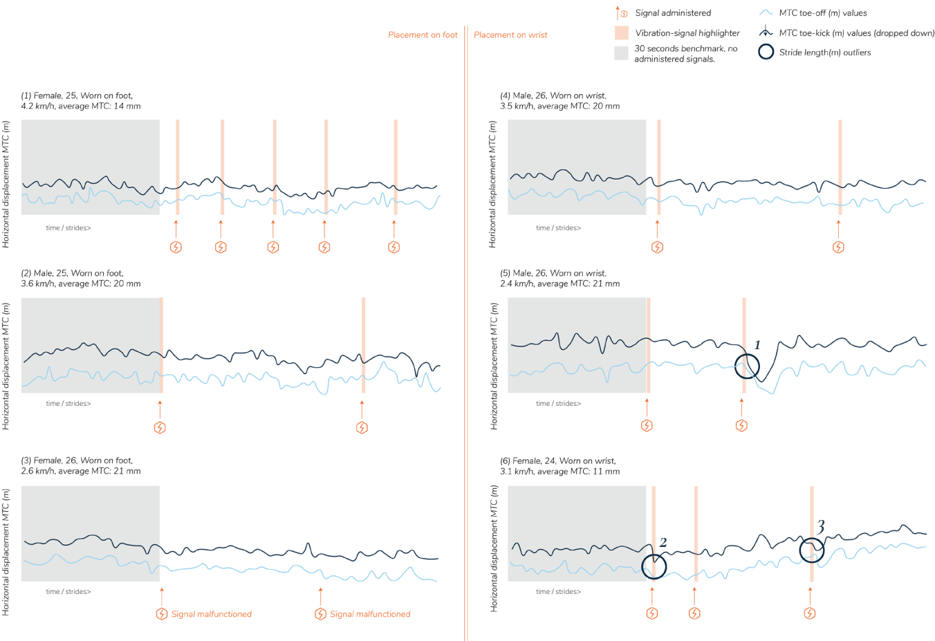
Figures 6.11(left) and 6.12(above): Vertical (left) and horizontal displacement (above) of the MTC for the six test subjects. The graphs containing the Tracker output data have been added to Appendix 12.
