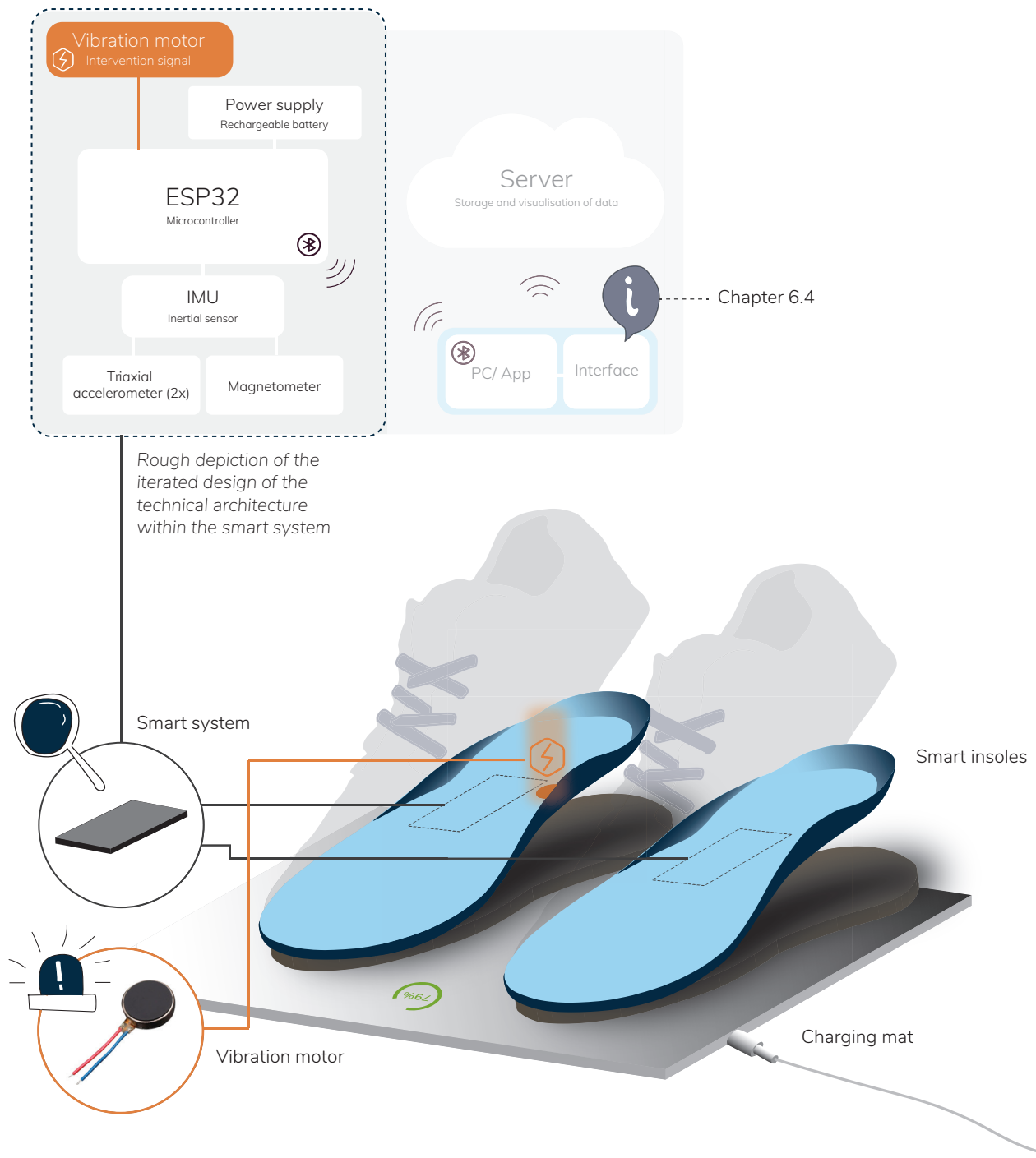
Figure 6.17: The concept-idea of the smart insoles with integrated intervention signal (the vibration motor)
