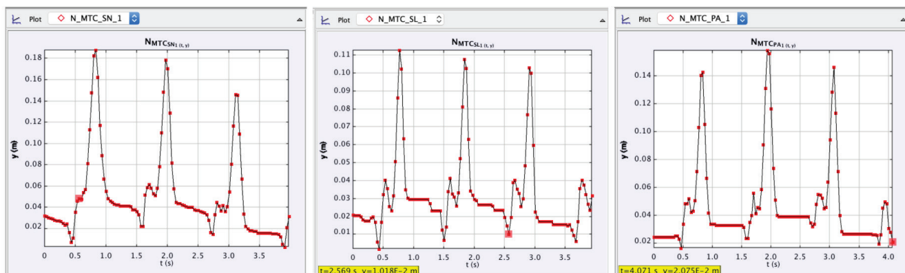
Figures 2.13-2.15: Vertical displacement of the MTC (or PTP) for three gait cycles for sneakers, flip-flops and soft slippers (l-r).
