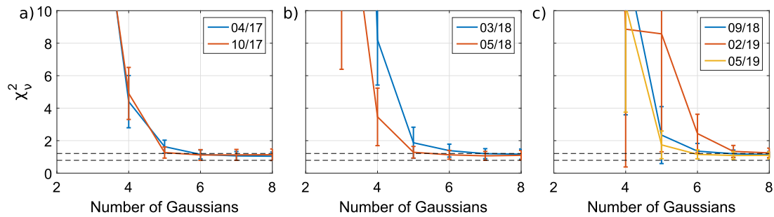
Fig. 7. Chi-square test applied to the seven MBES BS datasets. The solid lines and their error bars represent the mean and standard deviation of the reduced Chi-square values considering the incident angles from 40 to 65° of both the starboard and port sides. The black dashed line indicates a good model fit.
