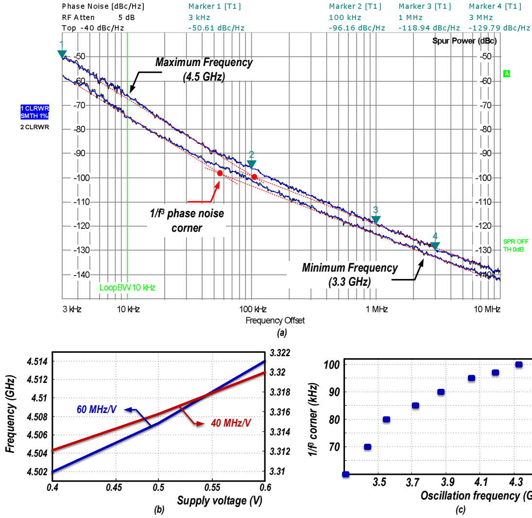
Figure 3.21: Class-D/ F_2 oscillator: measured (a) PN at f_{max} and f_{min} ; (b) frequency pushing due to supply voltage variation; and (c) 1/f^3 corner over tuning range.
