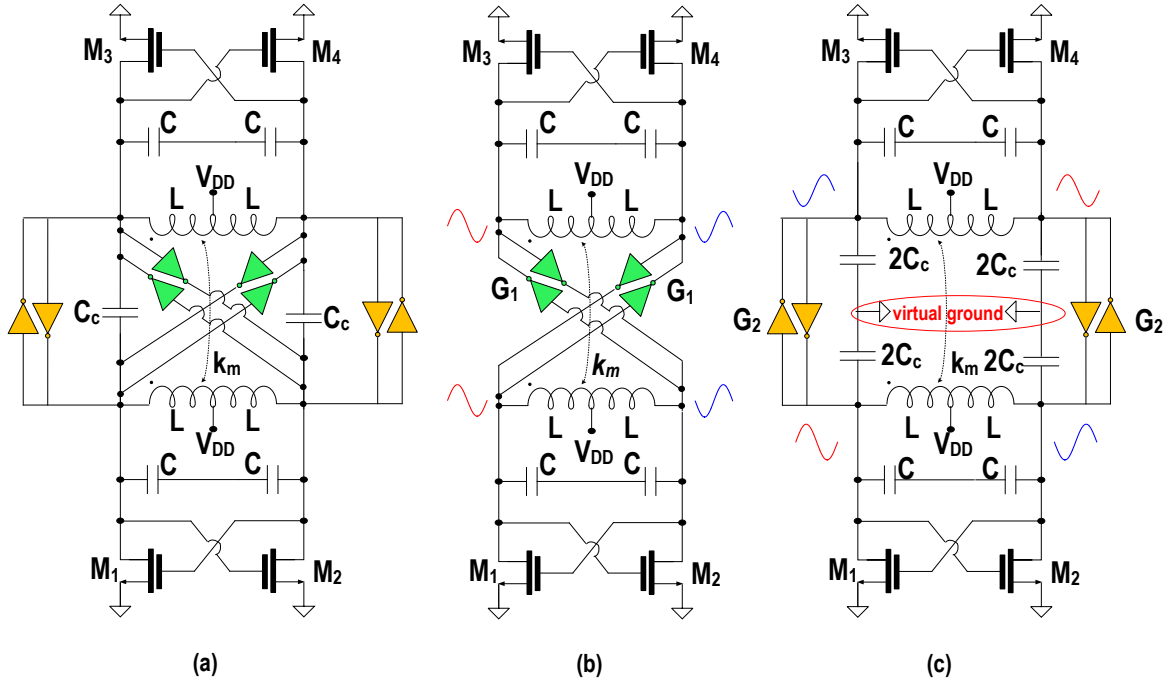
Figure 4.5: Differential trans-conductance schematic.
