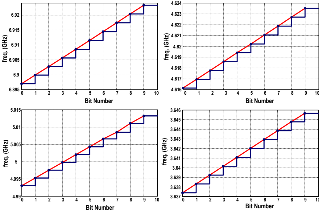
Figure 4.12: Acquisition bank linearity for different frequencies.
