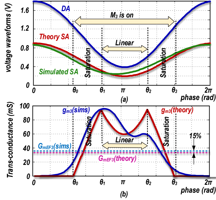
Figure 5.9: (a) Drain and source voltage waveforms. (b) g_{m3} : theory and simulations.
