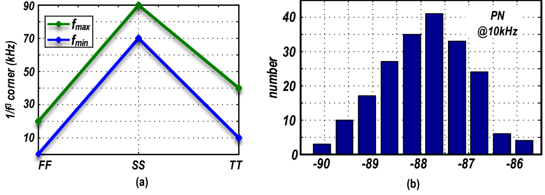
Figure 3.19: Class- F_{2,3} oscillator: 1/f^3 corner over process variation; and (b) histogram of PN at 10kHz offset frequency.
