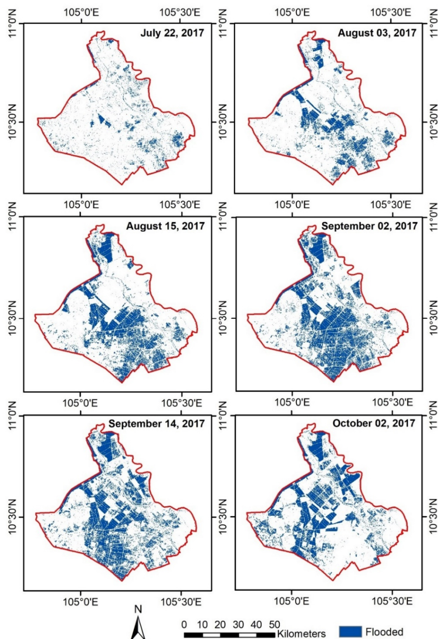
Figure 15. Flood extent maps during the flood event in 2017 using the change detection-based time series analyses on the derived surface water maps derived from the Sentinel-1 SAR data.
