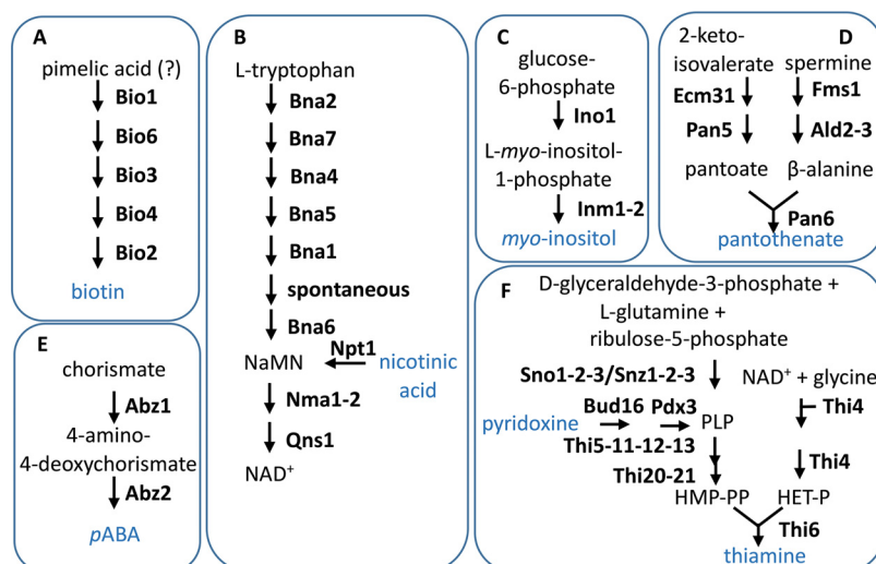
FIG 1 Schematic representation of the de novo biosynthetic pathways for the B vitamins biotin (A), nicotinic acid (B), myo -inositol (C), pantothenate (D), pABA (E), and pyridoxine and thiamine (F) in S. cerevisiae (5). Vitamins that are usually added to the chemical defined media for cultivation of yeasts are shown in light blue.
