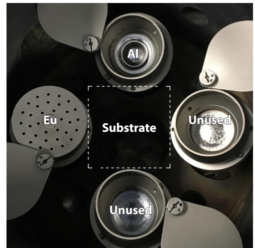
Fig. 2. Top-down photograph of the inside of the sputtering chamber, with the sources used for fabrication; the right and bottom sources are not used for fabrication.
