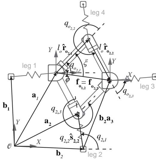
Figure D.1: An example of the various vectors that are used in the inverse kinematics and expressions of Jacobian matrices for mechanism III.
