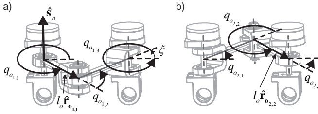
Figure E.3: a) the first end-effector serial chains and b) the second end-effector serial chain, which is also the third internal serial chain, both with examples of vectors and scalars that are used in the expression of the basis twists, the basis wrenches, and the inverse kinematics.
