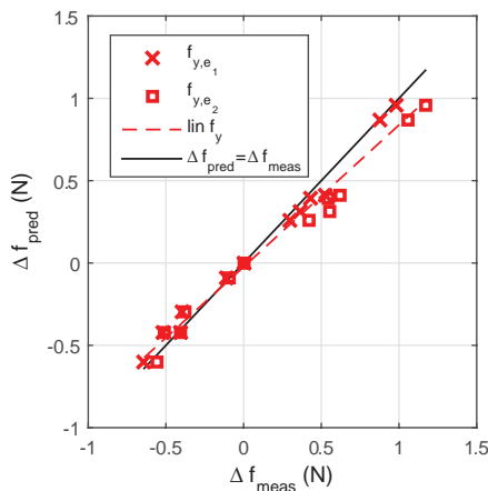
Figure 5.8: The correlation between the measured force values and those predicted using \mathbf{J}^{-\text{T}} at the poses listed in Table 5.1 along the axis in which the PM2E is constrained. A linear trend line is added around which the coefficient of determination are calculated.
