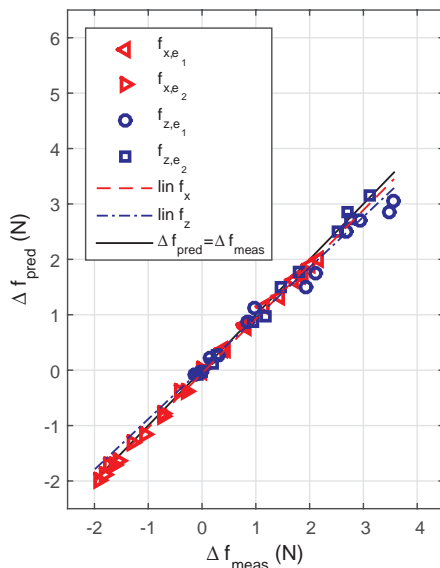
Figure 5.7: The correlation between the measured force values and those predicted using \mathbf{J}^{-\text{T}} at the poses as listed in Table 5.1 along the axes spanned by the DoFs of the PM2E. Linear trend lines are added around which the coefficients of determination are calculated.
