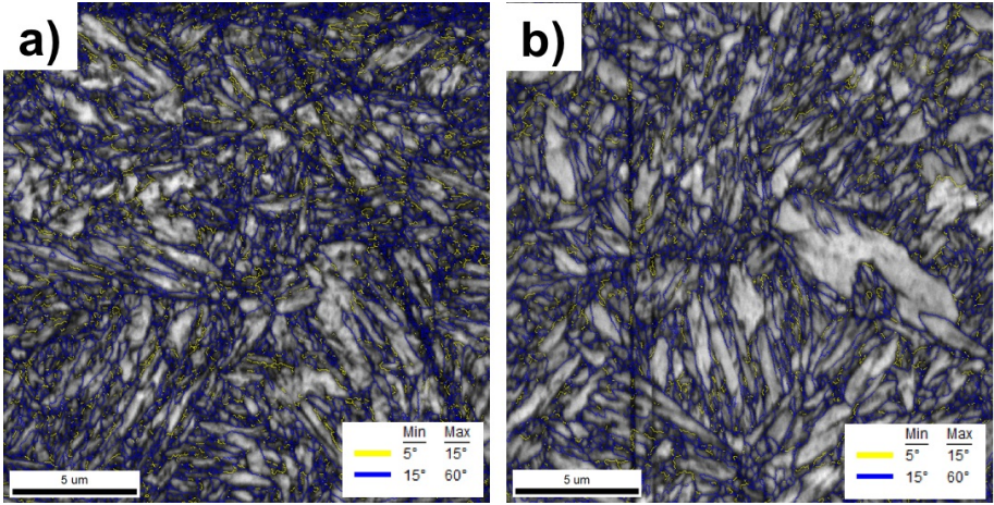
Figure 4.6: Image Quality EBSD maps of the tempered martensitic specimen. a) Surface. b) Bulk.
