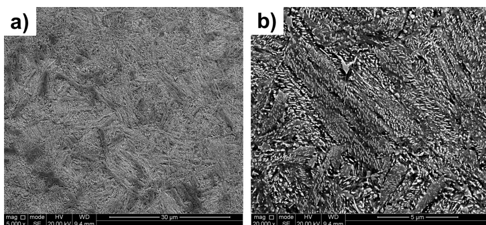
Figure 4.3: Scanning Electron Microscopy micrographs of lower bainitic microstructure.
