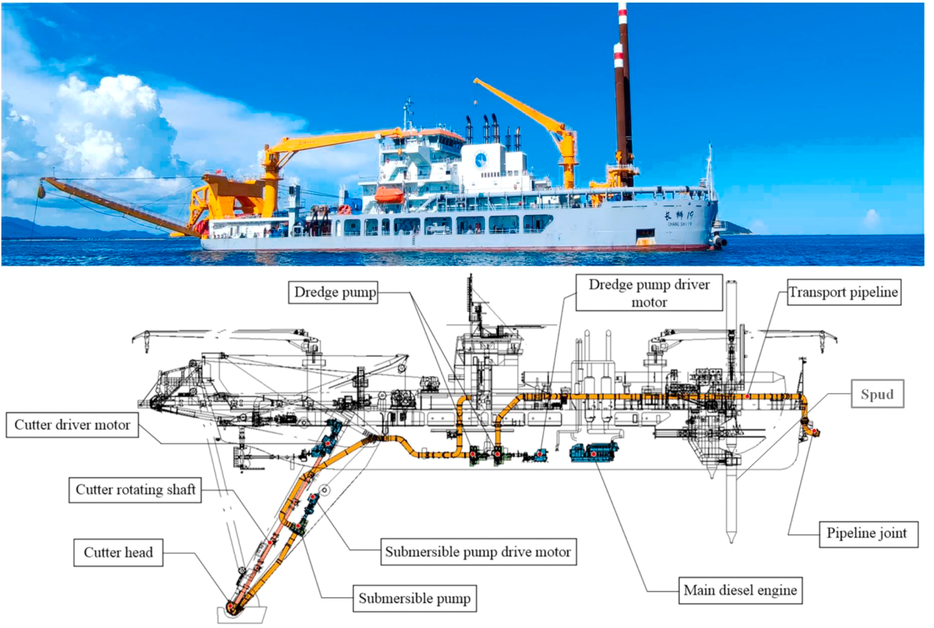
Fig. 1. “CHANGSHI 19” cutter suction dredger.
