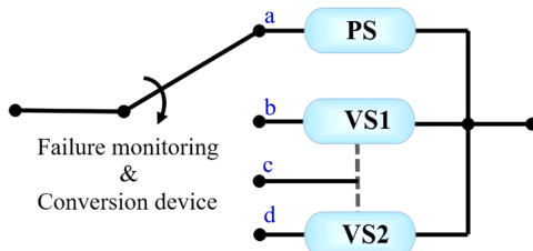
Fig. 4. Diagram of the hybrid redundancy sensor structure.
