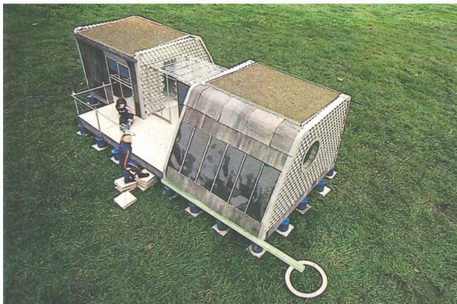
Fig. 10.5 Two-person dwelling, SUG, south-east side, pending wall with solar collectors. (Source: Kan 1978)
