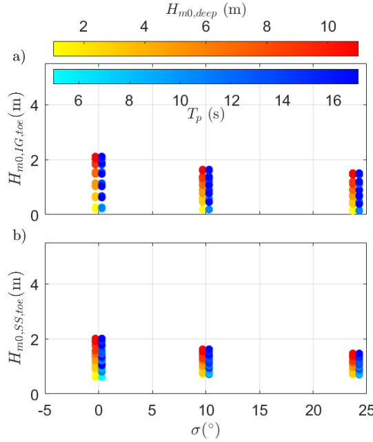
Figure 2.11. Scatterplots of a) H_{m0,IG,toe} and b) H_{m0,SS,toe} against \sigma ( h_{toe} = 1 m, \cot(m) = 50 , W_{veg} = 0 m, n = 0.012 s/m 1/3 and \cot(\alpha) = \infty ). Each data point is represented by two markers with colormaps indicating the magnitude of H_{m0,deep} (hot) and T_p (cold).
