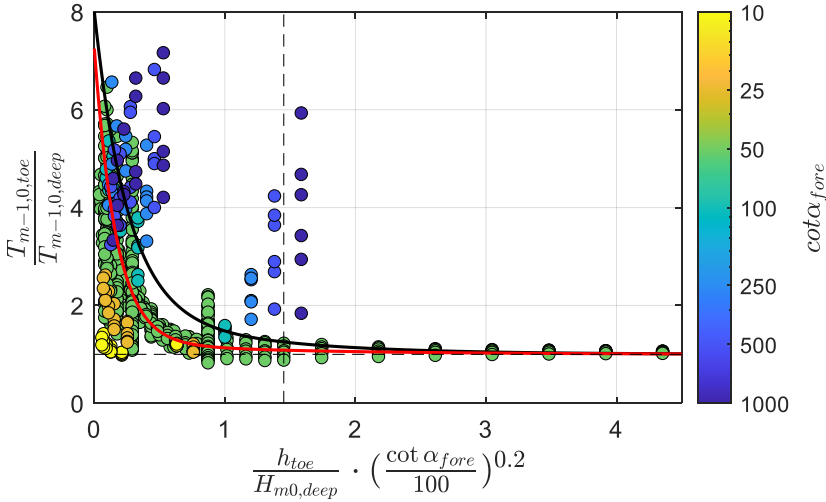
Figure D. 1 Numerically modelled realtive spectral wave period as a function of relative water depth and foreshore slope, following Hoiland et al. (2017). Black and red lines represent Equations C.1 and C.2, respectively.
