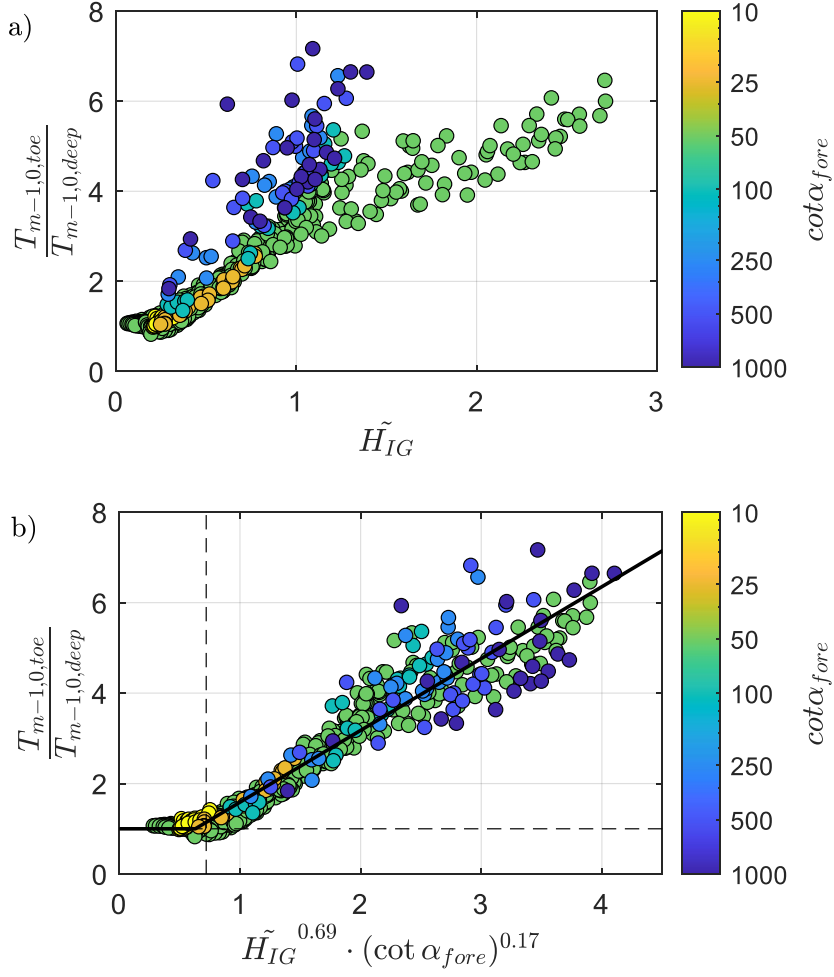
Figure D. 2 Numerically modelled realtive spectral wave period as a function of a) \tilde{H}_{IG} alone; and b) \tilde{H}_{IG} and an additional foreshore-slope term. Solid line represents Equation D.4. Dashed vertical line indicates h_{toe}/H_{m0,deep} = 1 and dashed horizontal line represents the deep-water limit where T_{m-1,0,toe}/T_{m-1,0,deep} \approx 1 .
