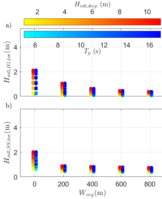
Figure 2.19. Scatterplots of a) H_{m0,IG,toe} and b) H_{m0,SS,toe} against W_{veg} ( \sigma = 0^\circ , h_{toe} = 1 m, \cot(\alpha) = 50 , n = 0.012 s/m 1/3 and \cot(\alpha) = \infty ). Each data point is represented by two markers with colormaps indicating the magnitude of H_{m0,deep} (hot) and T_p (cold).
