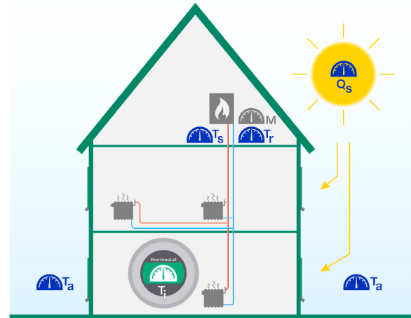
Fig. 1. Schematic of the experimental set-up for the dynamic integrated co-heating test of individual buildings. The gas heater is equipped with temperature sensors ( T_s , T_r ) and a flow meter ( m ). The indoor temperature ( T_i ) is monitored with the central thermostat. Ambient temperature ( T_a ) and solar influx ( Q_s ) are obtained from nearby weather station.
