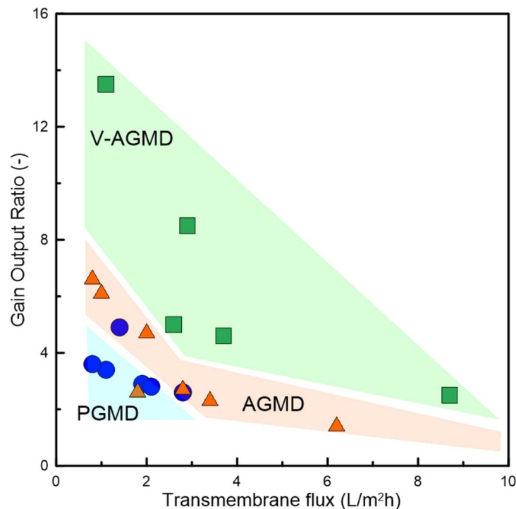
Figure 7. GOR vs transmembrane flux in AGMD, vacuum-enhanced AGMD (V-AGMD), and permeate gap membrane distillation (PGMD). Data from [75].
