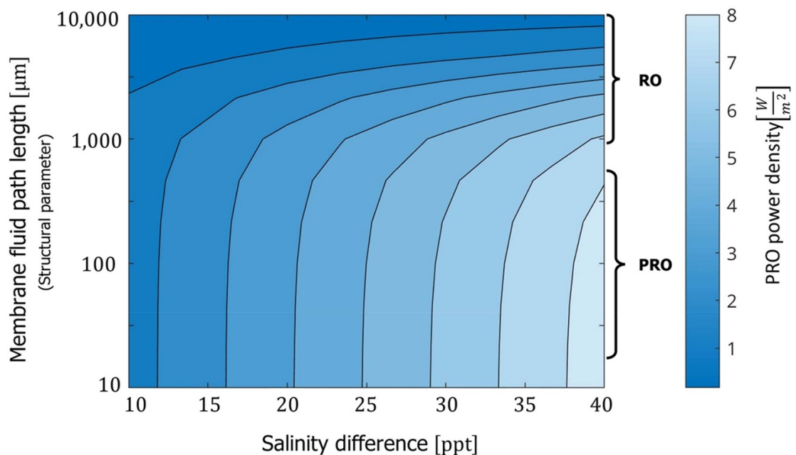
Figure 14. Structural parameter and salinity difference as a function of power density. Increasing the salinity difference applied at the feed and draw while decreasing the structural parameter increases the PRO power density. The labels for RO and PRO highlight the variation of structural parameter found in existing membranes. Reprinted from [219], Copyright (2021), with permission from Elsevier.
