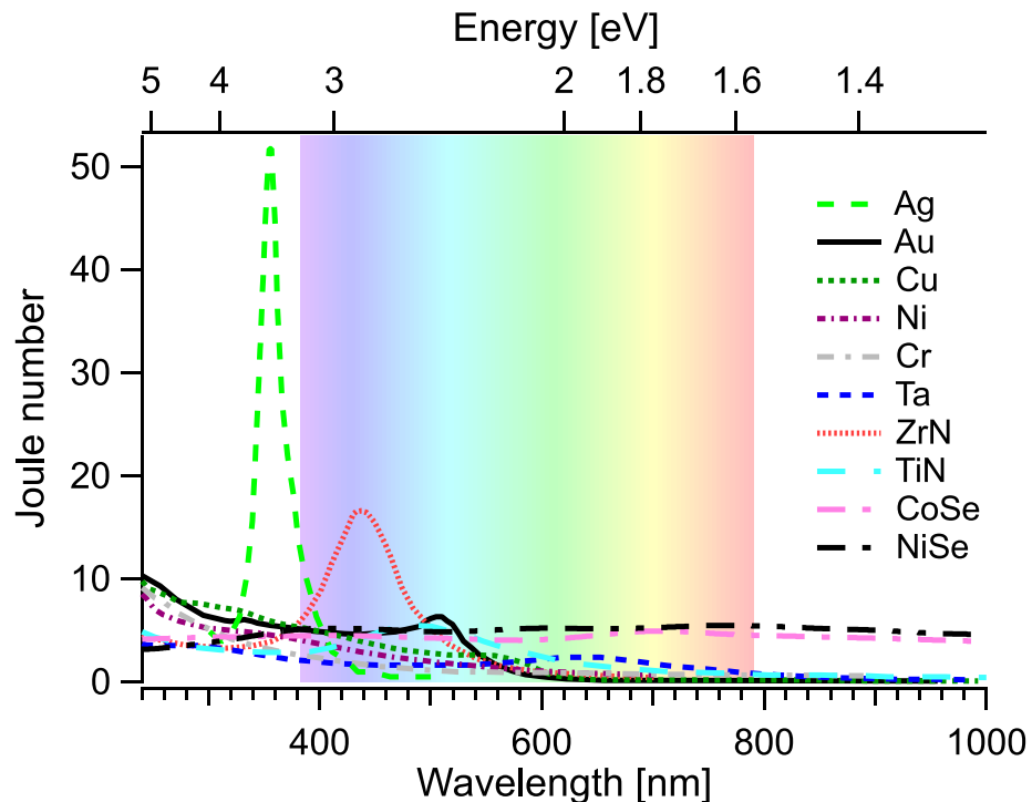
Figure 8. Joule number J_0 for different metals: Ag, Au, Cu, Ni, Cr, Ta, ZrN, TiN (data taken from [133]), CoSe, NiSe (data taken from [106]).
