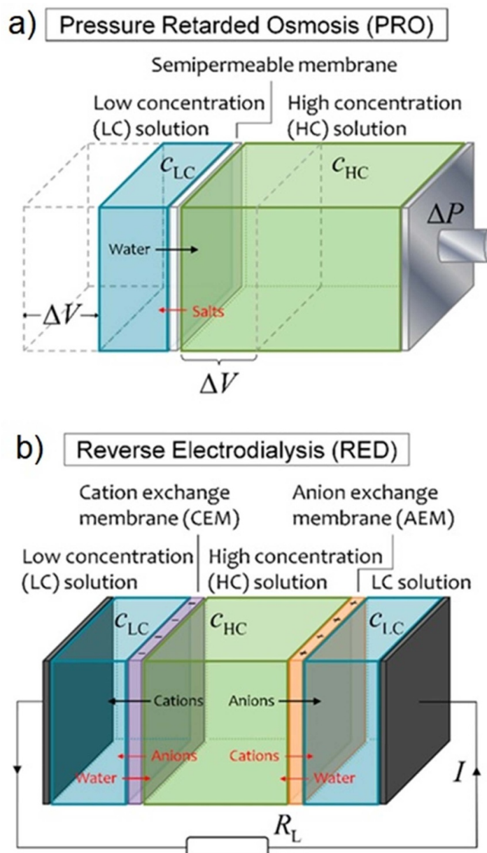
Figure 12. Schematic (a) represents the PRO where the salinity gradient produces the osmotic driving force for water flux from the feed (LC) to the draw (HC). (b) Represents the RED where the concentration difference across the IEM produces an electrochemical potential that allows the exchange of counter ions. Reprinted with permission from [213]. Copyright (2014) American Chemical Society.
