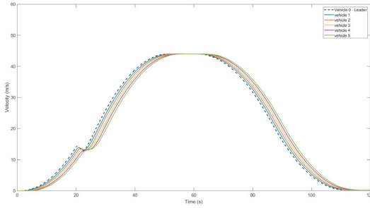
Fig. 2. No saturation with standard control: velocity response.
