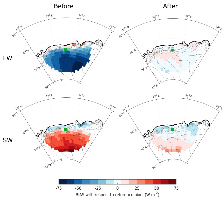
Figure 7. Yearly mean bias for each 2^\circ by 1^\circ grid box with respect to the centre pixel in which the AWS is located, before and after spatial correction for the example of PE, Antarctica (indicated by the green square). These results are based on all 2B-FLXHR-LIDAR data from 2007 to 2010 within a distance of 1000 km from the station. It should be noted that the comparison before spatial correction here has also been masked for ocean and different surface albedos.
