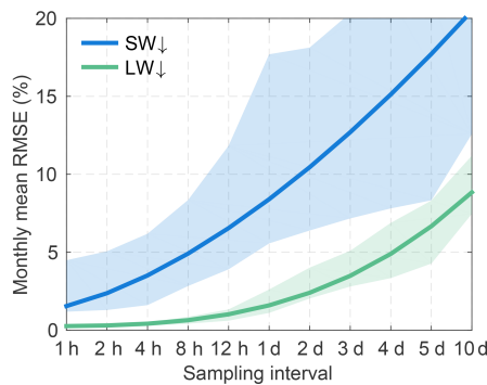
Figure 4. Monthly mean SW↓ and LW↓ RMSE (%) in function of sampling interval as derived from six AWSs. The RMSE was calculated by comparing the monthly mean estimates based on a sub-sample of data with a specified sampling interval to the full hourly datasets. The two curves represent the average relationship, while the shaded areas indicate the range for the different stations. Observation times range from 2007 to 2010, although with varying availability for the different AWSs.
