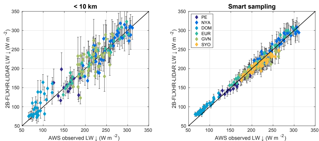
Figure 9. Monthly mean \text{LW}\downarrow radiation comparison between 2B-FLXHR-LIDAR and AWS (2007–2010). Based on retrievals comprising of all satellite samples < 10 km from station ( r = 0.94 ) (left). Based on all satellite samples resulting from the smart sampling approach ( r = 0.99 ) (right).
