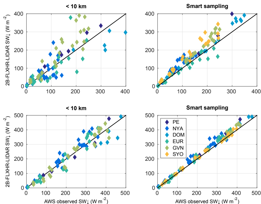
Figure 12. Monthly mean SW\downarrow radiation comparison between 2B-FLXHR-LIDAR and AWS (2007–2010). Based on retrievals comprising of all satellite samples < 10 km from station, P10 ( r = 0.85 ) (upper left). Smart sampling approach, P10 ( r = 0.97 ) (upper right). Retrievals < 10 km from station, P90 ( r = 0.96 ) (lower left). Based on all satellite samples resulting from the smart sampling approach, P90 ( r = 0.99 ) (lower right).
