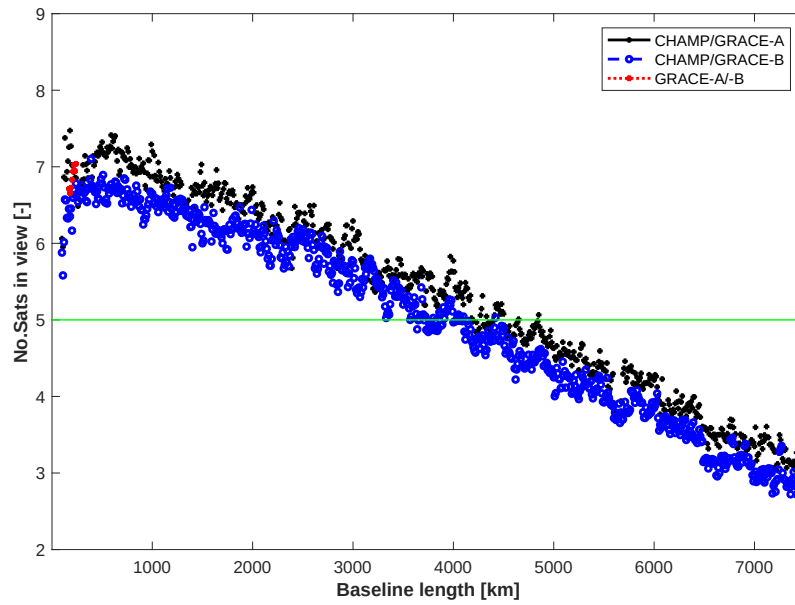
Figure 2: The number of GPS satellites simultaneously tracked by two space-borne GPS receivers as a function of distance (every 10 km) for each dual-satellite pair (analysis for 30 24-hr orbital arcs).
