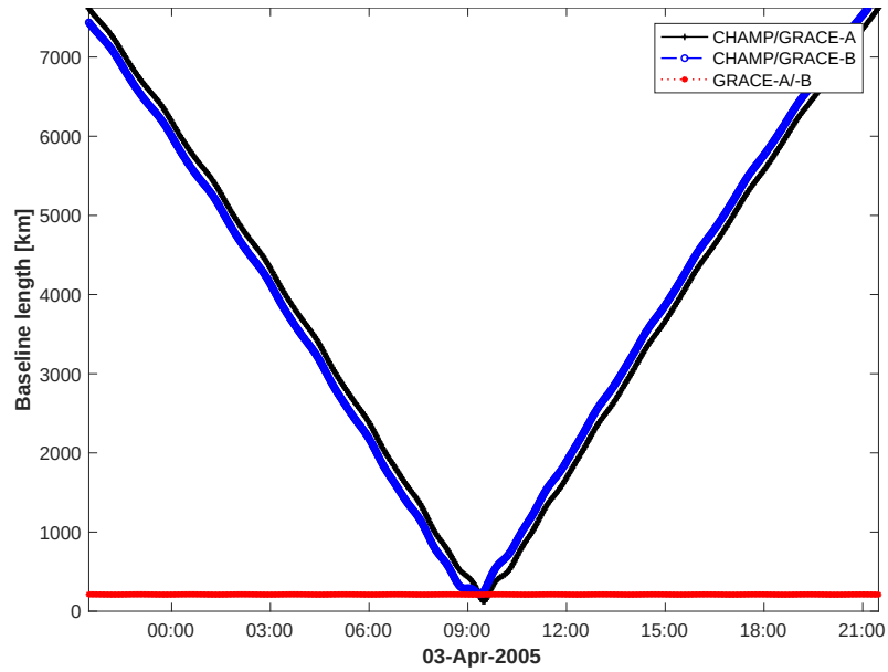
Figure 1: Baseline length variations for each dual-satellite pair during a representative 24-hr orbital arc (DOY 093, 2005). The GRACE baseline has been stabilized at around 220 km, the two CHAMP/GRACE baselines are rapidly changing from 110 to 7500 km in 24 hours.
