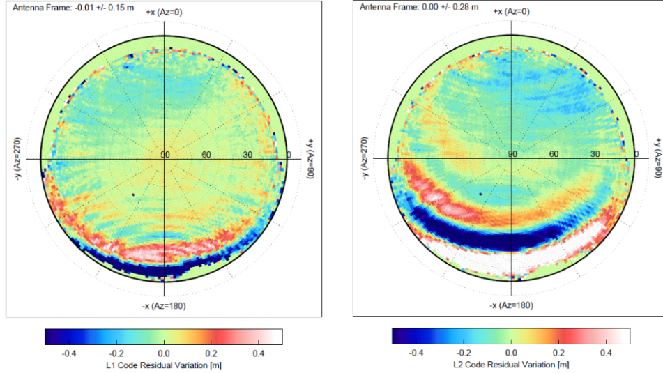
Figure 5: The CHAMP GPS receiver code residual variation patterns on the first (left) and the second (right) GPS frequency in the antenna-fixed reference system, for which the North axis coincides with the satellite body-fixed +X axis ( 0^\circ azimuth), the Up and bore-sight axis coincides with the -Z axis, and the East axis completes the right-handed system. The April 2005 (DOY 091-120) data were used for generating the CRV maps.
