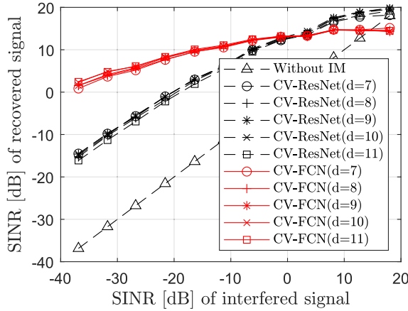
Fig. 8. Performance comparison of the CV-FCNs with CV-ResNets, where d means the number of convolutional layers in the network.
