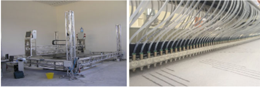
Fig. 2.14 D Shape® 3D-printer (left) and print head (right) (Lowke et al. 2018)
