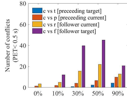
(a) Reactive ADS at low on-ramp demand
