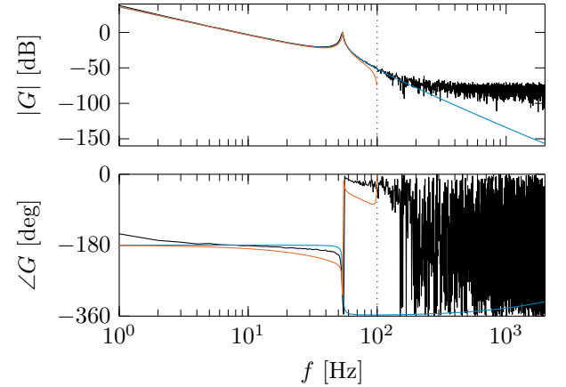
Fig. 6. Bode diagram of experimental setup: frequency response data (—), continuous-time model G_c (—), and discrete-time model G_d (—). Nyquist frequency is shown in a black dotted line (···).
