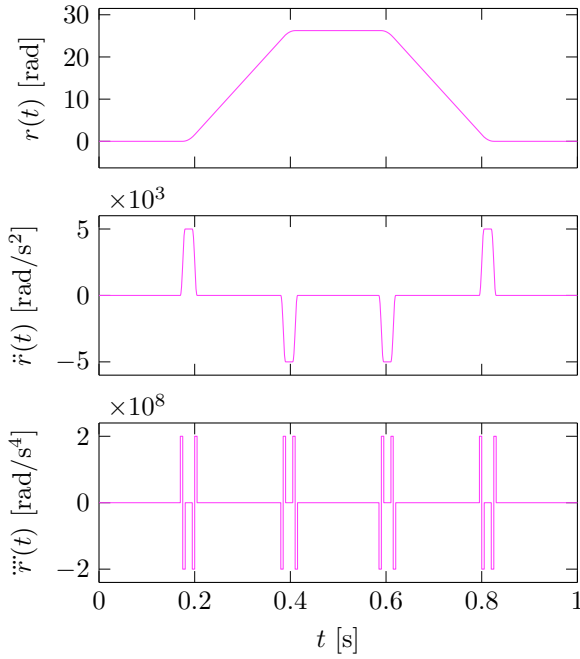
Fig. 7. Continuous-time 4 th order polynomial trajectory reference: position r(t) , acceleration \ddot{r}(t) , and snap \dddot{r}(t) .
