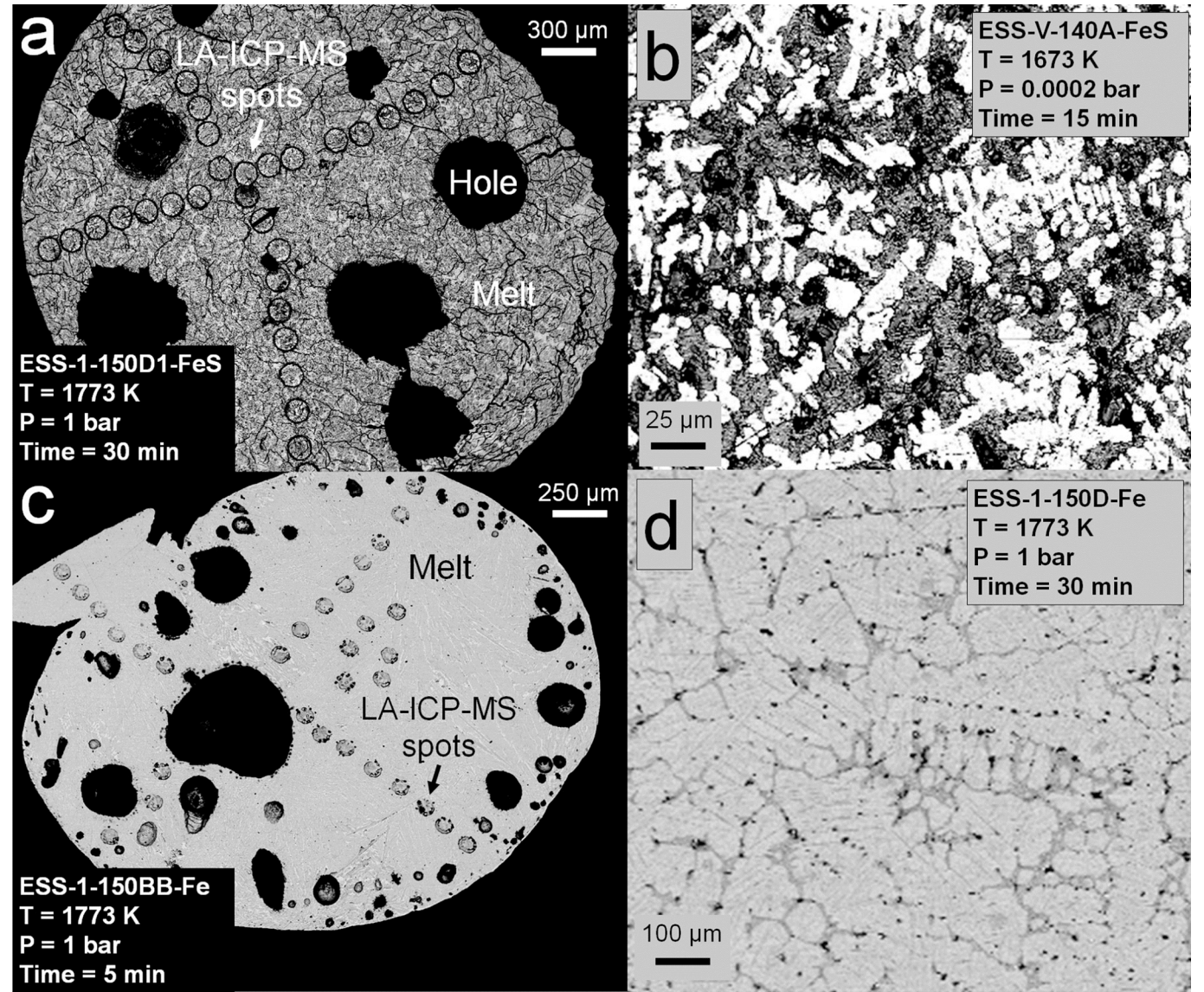
Fig. 1. Backscattered electron images of FeS and Fe samples. Panel (a) shows an overview of a typical FeS experimental run product, ESS-1-150D1-FeS, conducted at 1 bar and 1773 K for 30 min. Clearly visible are the LA-ICP-MS spot pits placed from rim to rim. Panel (b) depicts the FeS melt texture observed for run ESS-V140A-FeS, conducted at 1673 K, vacuum (0.0002 bar) for 15 min. This texture was found to be typical for experimental samples that experienced significant S loss, resulting in the separation of FeS-rich (dark) and FeS-poor (white) melts. Panel (c) shows an example of a typical Fe metal run product and panel (d) quench textures observed in the Fe melt of run ESS-1-150D-Fe.
