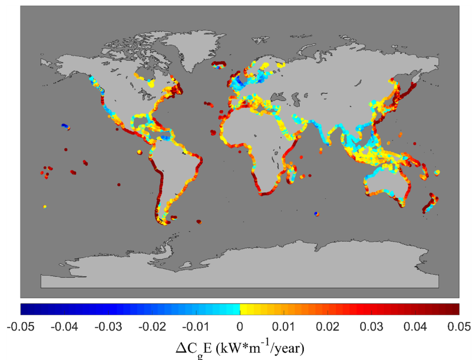
Figure 1. Global distribution of trend in annual average values of wave energy flux, \Delta C_g E (\text{kWm}^{-1}/\text{year}) at sandy beach locations for the period of 1984–2016 from the Liu et al. 33 dataset [Map generated using Matlab Mapping toolbox].
