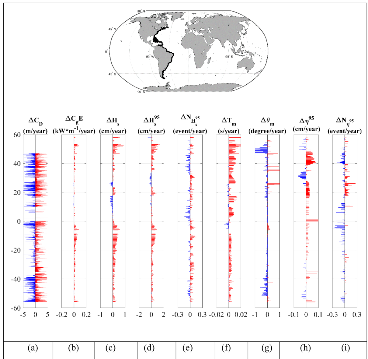
Figure 5. As for Fig. 4 but for the east coast of North and South America.
