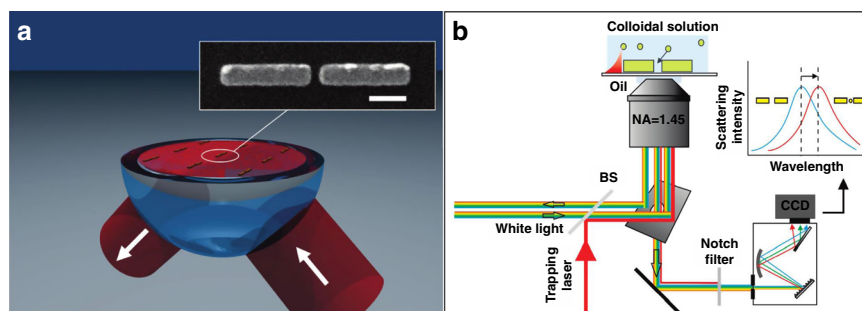
Fig. 5 Principle of structural plasmonic tweezers. a Surface plasmonic trapping configuration through the design of nanostructures, scale bar: 200 nm. b Experimental configuration. The trapping events can be directly monitored using scattering spectra of the antennas. a Reproduced with permission from ref. 281 , Copyright 2009, American Chemical Society. b Reproduced with permission from ref. 86 , Copyright 2010 American Chemical Society
