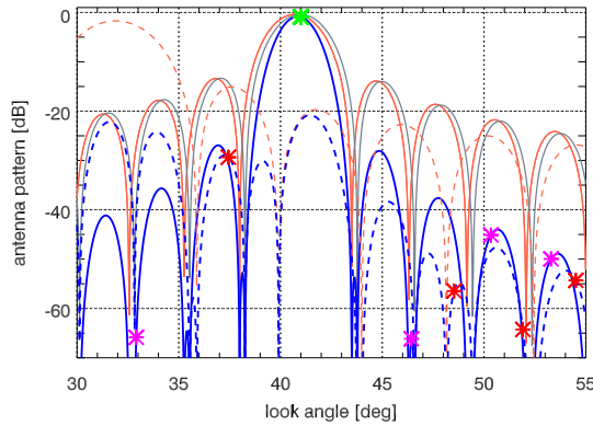
Fig. 5. Elevation patterns involved in the imaging of the eighth subswath (solid lines: patterns related to the imaged subswath; dashed lines: with the coupled subswath; orange lines: Tx, gray lines: Rx, and blue lines: two way). The position of the useful signal and ambiguous signals are marked by an asterisk (green: signal and red/magenta: ambiguities of odd/even order).
