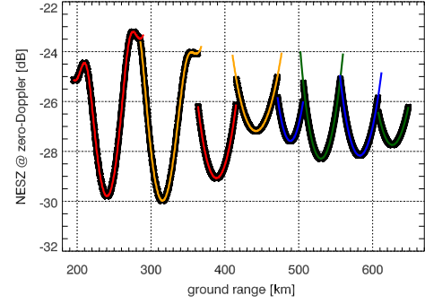
Fig. 3. NESZ computed at zero Doppler versus ground range.
