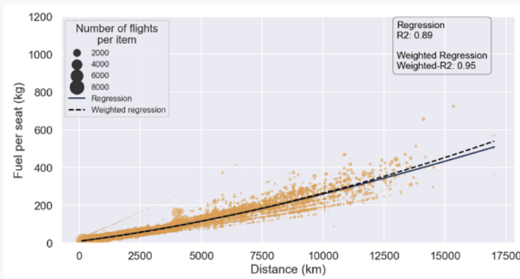
Figure 2. Weighted regression, improvement to article Fig.5
