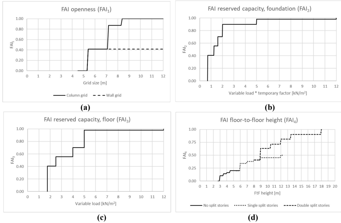
Figure 2. Relation between FAI and design factors a: Openness ; b: Reserved capacity foundation ; c: Reserved capacity floor ; d: Floor-to-floor height.
