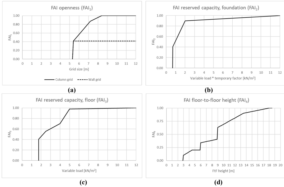
Figure 3. Smoothened FAI for a: Openness ; b: Reserved capacity foundation ; c: Reserved capacity floor ; d: Floor-to-floor height.
