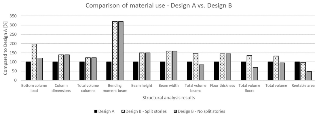
Figure 4. Comparison material use between Design A and B, normalized such that Design A is 100%.
