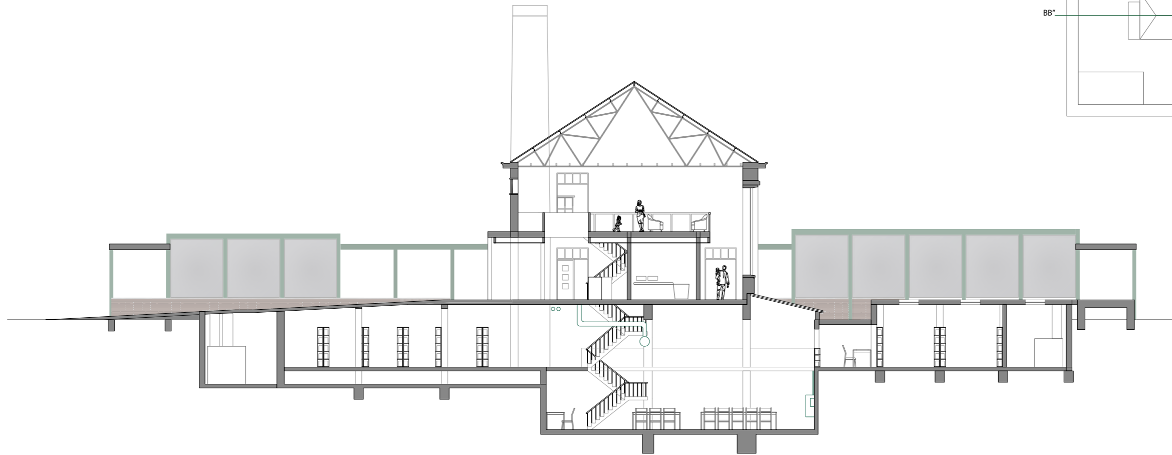
Section AA''
