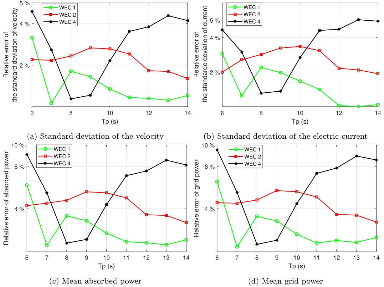
Fig. 7. The relative errors of the proposed SD model to the TD model across various peak periods. ( H_s = 2 m and B_{pro} = 100 kNs/m).
