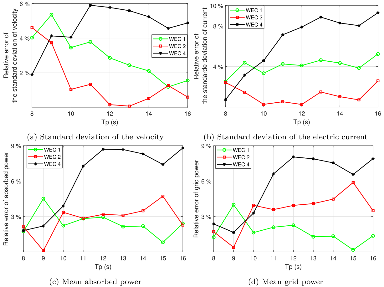
Fig. 16. The relative errors of the proposed SD model to the TD model for the array layout 3 across various peak periods. ( H_s = 4 m and B_{p10} = 100 kNs/m).
