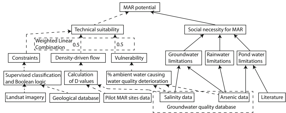
Fig. 2 Methodological framework to determine potential for MAR, combining spatial distributions of social necessity and technical hydrogeological feasibility. The ‘D value’ is a dimensionless indicator for the impact of density-driven flow (Bakker 2010)
