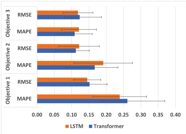
Fig. 10. Averaged RMSE and MAPE results models for different objectives
