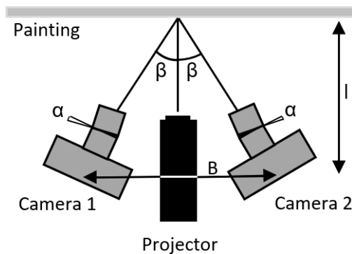
Figure 2: The setup of fringe encoded stereo imaging as seen from a top view. The cameras are placed 200 mm ( l ) from the painting with 140 mm ( B ) spacing between the cameras. The optical axis of the cameras relative to the painting's normal vector is 21.5^\circ ( \beta ). The tilt-shift lenses are tilted by 8^\circ ( \alpha ) to align the focal plane with the painting's surface.
