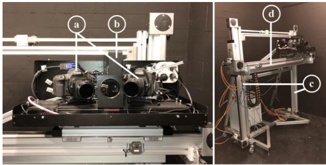
Figure 3: The XY-stage translates (a) the two cameras and (b) projector parallel to the painting, (c) two vertical linear drivers and (d) a horizontal linear driver provide the precise, automated movement, while minimizing the vibrations with a rigid structure.
