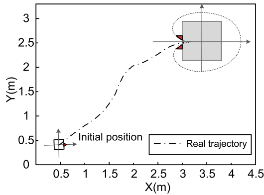
Fig. 13. The trajectory of the Chaser.
