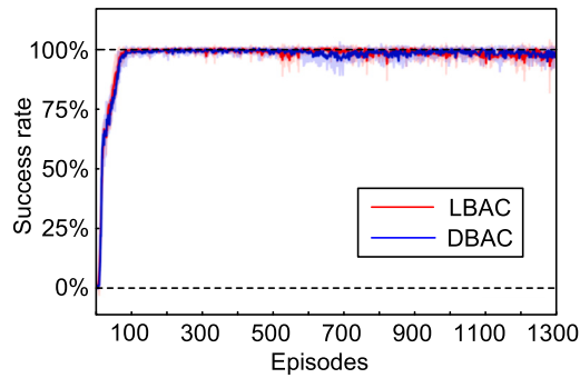
Fig. 8. The success rate during training.
