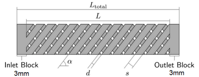
Fig. 1. The geometry and parameters of the reactor. Shown is the effective interior volume, i.e. the volume taken up by the fluid; the gaps are the space taken up by the mixing elements.
