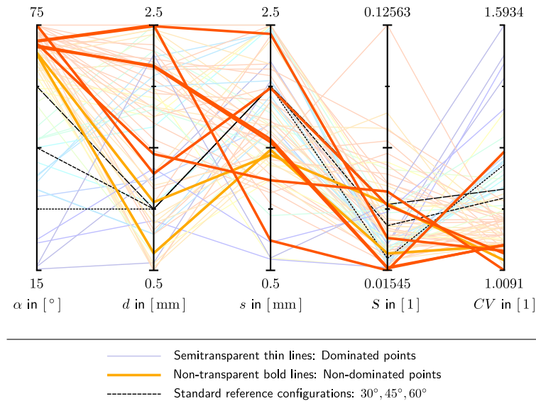
Fig. 4. Parallel coordinates plot for \alpha, d, s (cf. Fig. 1) and the objectives S and CV . Every line in the plot corresponds to one simulated configuration, with color corresponding to the mixing bar angle \alpha .
