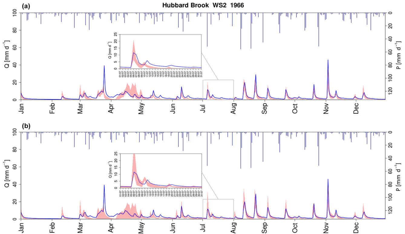
Figure 10. Hydrograph of Hubbard Brook WS2 with the observed discharge (blue) and the modelled discharge represented by the 5/95% uncertainty intervals (red), obtained with (a) a constant representation of the root-zone storage capacity S_{u,max} and (b) a time-varying representation of the root-zone storage capacity S_{u,max} . Blue bars indicate precipitation.
