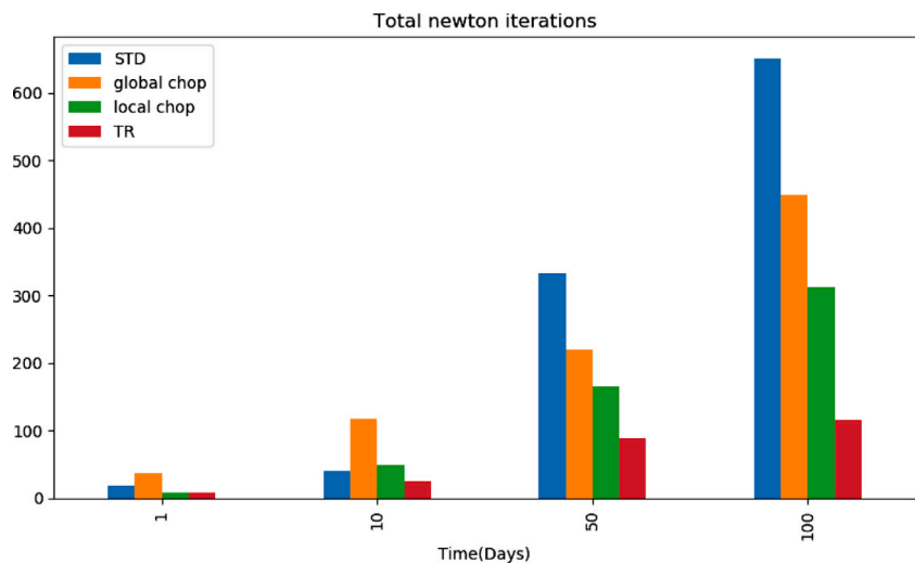
Fig. 15. Comparison of cumulative Newton iteration for different nonlinear solver for egg-model at different time.
