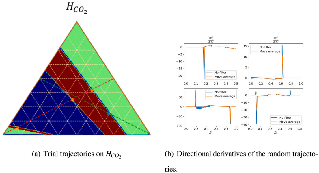
Fig. 5. Full and directional evaluations of second order behavior for ternary compositional kernel.
