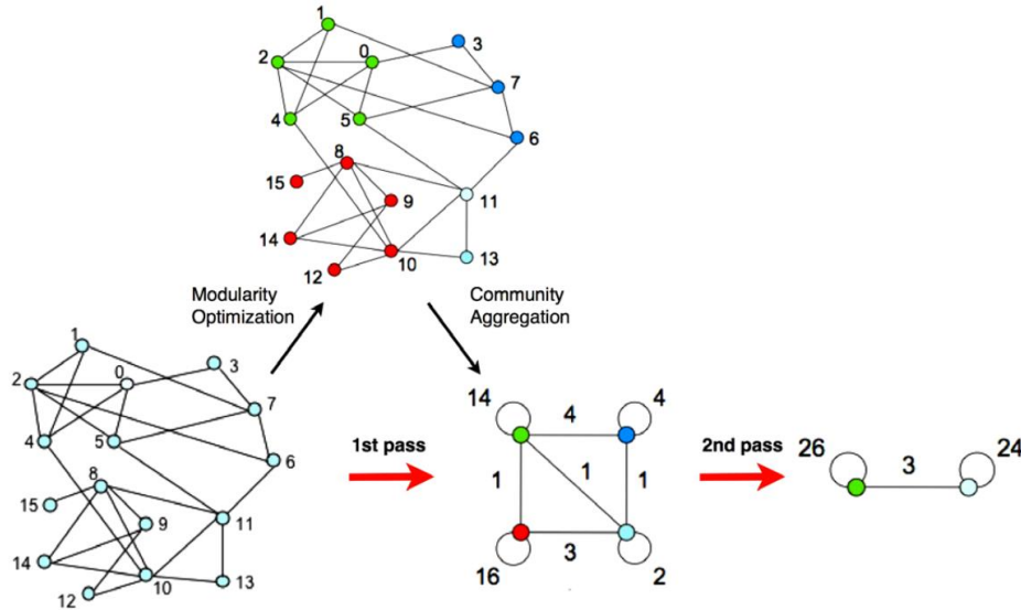
Figure 4. Visualization of the steps of the Louvain method. Each pass consists of two phases. In the first phase, the modularity is optimized by allowing only local changes of communities; in the second one, the communities found are aggregated in order to build a new network of communities. The passes are repeated iteratively until no increase in modularity is possible (Blondel et al. (2008)).
