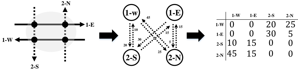
Figure 3. Illustration of the topological representation for the hub transfer pattern. The original layout of the identified hub (shaded area) is presented on the left with four directed lines marked, i.e. 1-E, 1-W, 2-S and 2-N. The transfer pattern is then represented as a graph (middle). The weighted adjacency matrix is displayed on the right.
