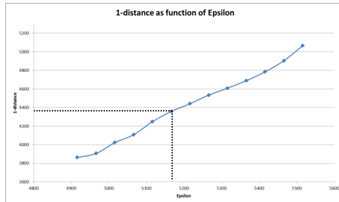
Figure 6. 1-distance plot as function of \epsilon
