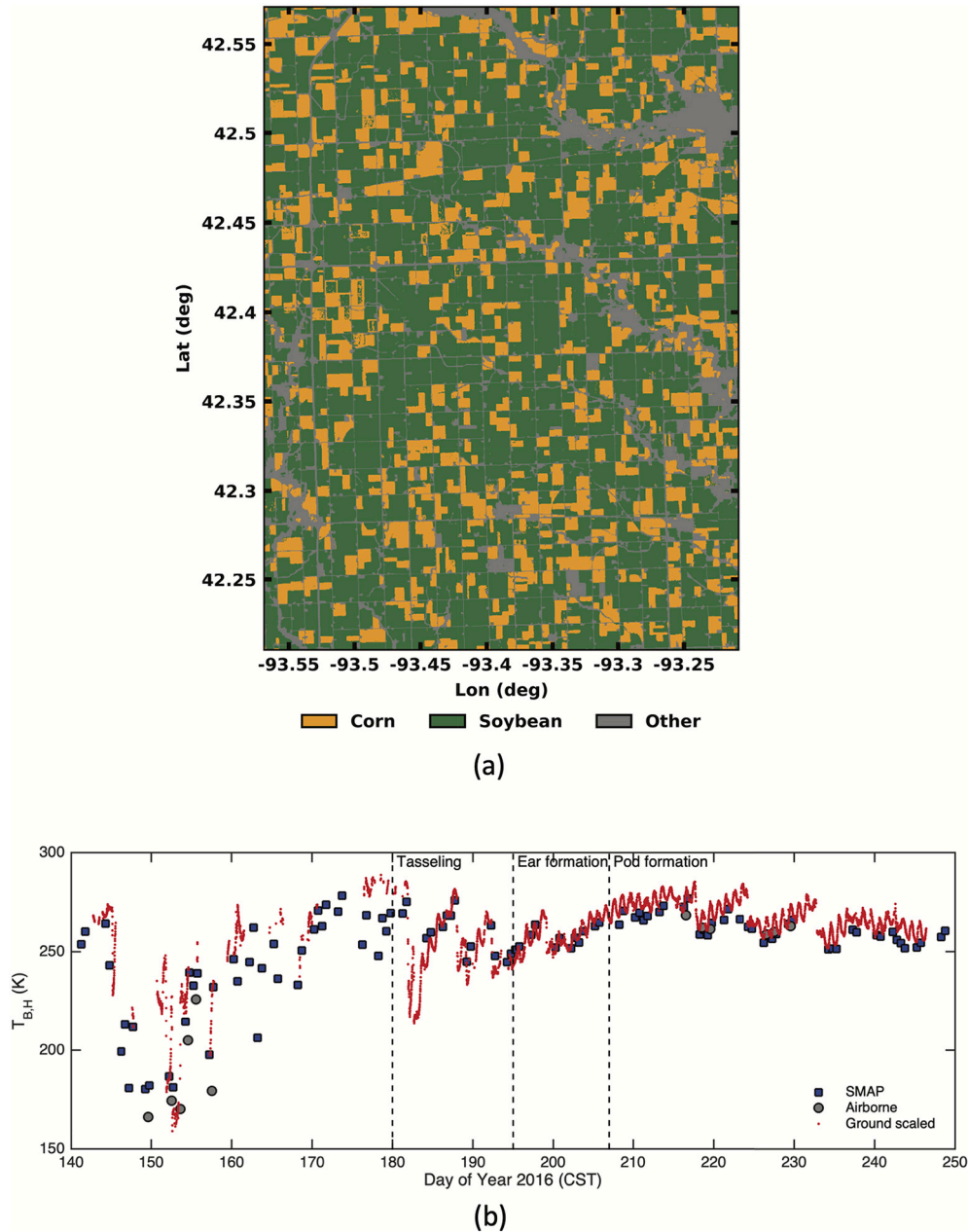
Fig. 7. (a) Land cover fraction in the 36 km SMAP pixel from the US Department of Agriculture (USDA) Crop Data Layer (CDL) (USDA, 2016) and (b) Upscaled ground-based H-pol T_B compared with the SMAP and the PALS observations at 36 km.
