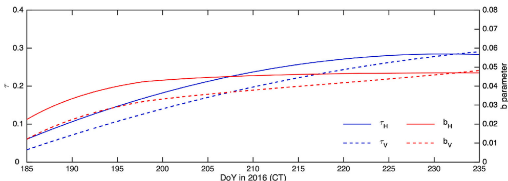
Fig. 9. Optimized vertical and horizontally polarized vegetation opacities, \tau_H and \tau_V , respectively, obtained from the microwave emission model at the corn site during SMAPVEX16-MicroWEX.
