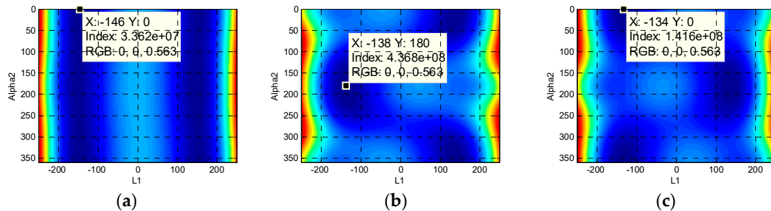
Figure A2. Part of simulation verification of numerical optimization with fixed A_2 . The corresponding parameters are: (a) A_2 = 50, i_c = 8^\circ ; (b) A_2 = -200, i_c = 12^\circ ; (c) A_2 = 150, i_c = 16^\circ .
