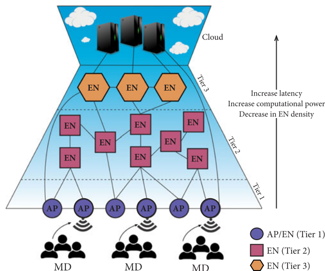
Fig. 2. Multi-tier edge-cloud infrastructure.
