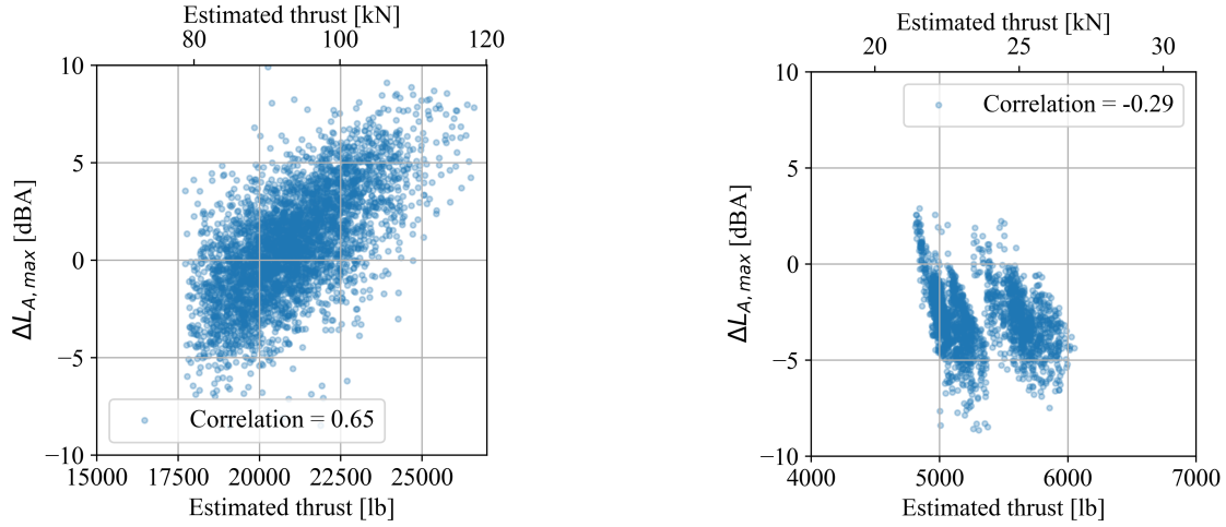
(a) Differences in L_{A,max} for departure procedures.
