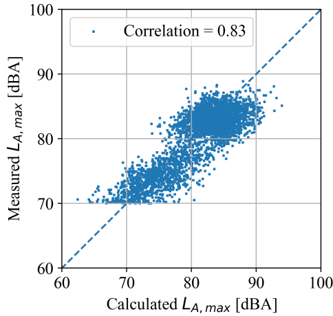
(a) Schiphol departure measurements compared to model results.
