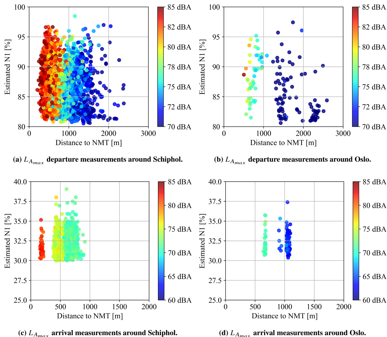
Fig. 4 Sound level of measurements of B737-800 with respect to distance and N1\% for the baseline (AMS) and verification (Oslo) dataset.
