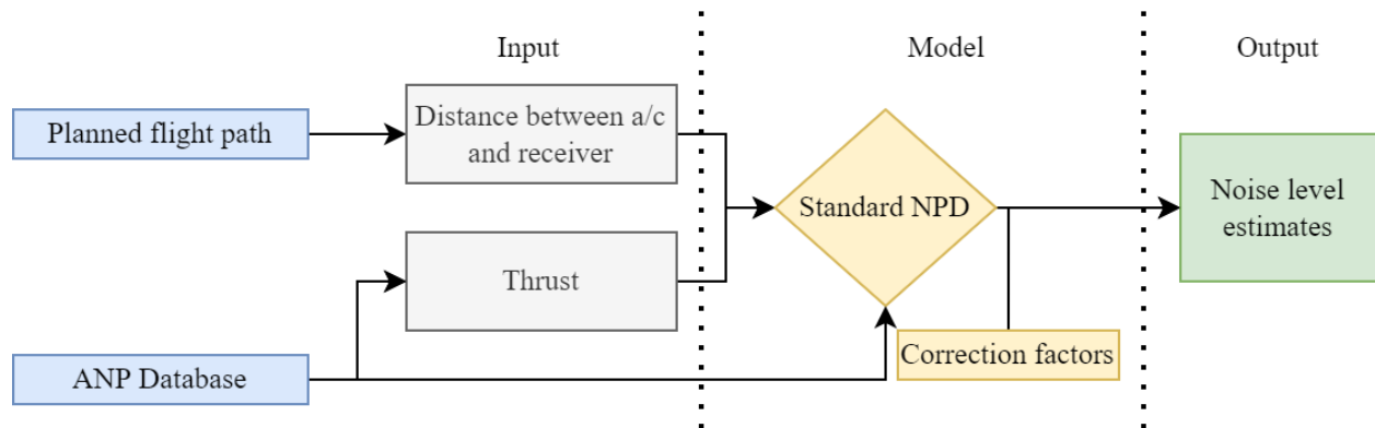
Fig. 1 Flowchart of input and output of the Doc.29 aircraft noise model.
