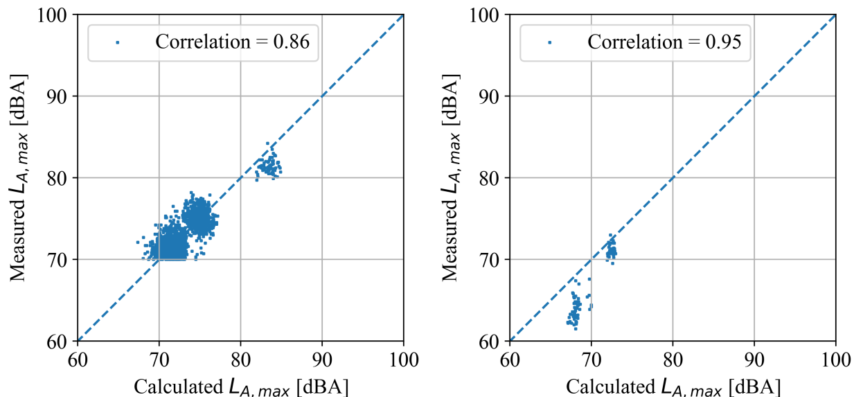
(a) L_{A,max} Schiphol calibration data set using new NPD tables. (b) L_{A,max} Gardermoen verification data set using new NPD tables.
