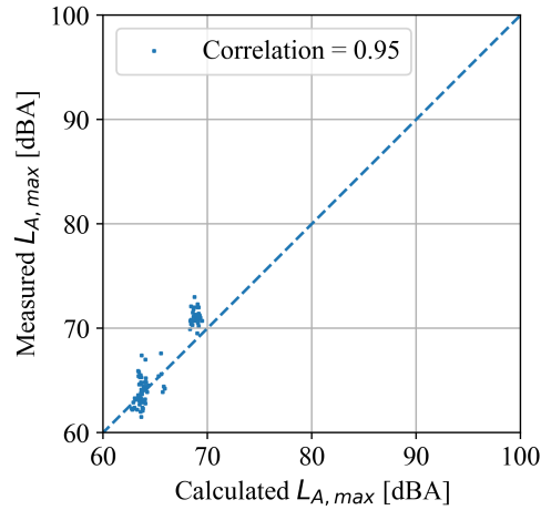
(c) Schiphol arrival measurements compared to model results.
