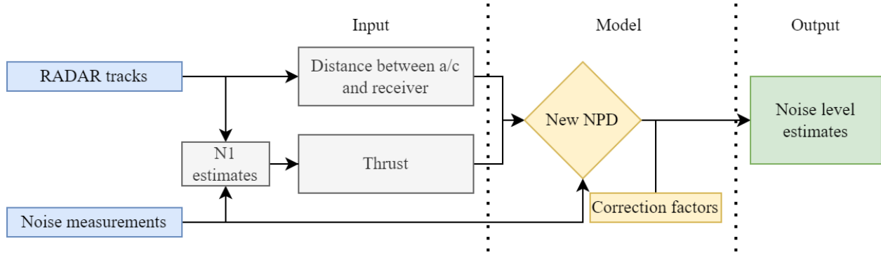
Fig. 11 Flowchart of new method of Doc.29 noise calculations
