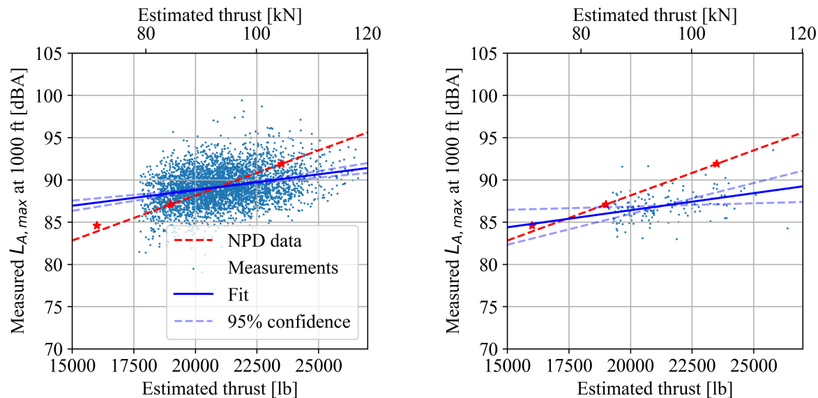
(a) Schiphol departure measurements standardised for 1000 ft. (b) Oslo departure measurements standardised for 1000 ft. Taken from [9].
