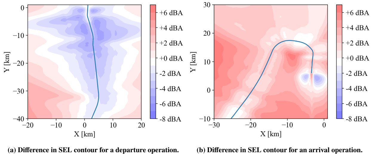
Fig. 10 Difference in SEL contours between baseline and calibrated models.
