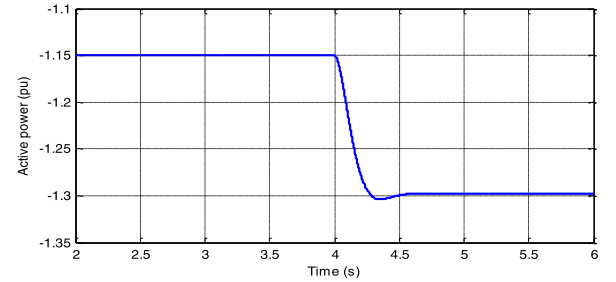
Fig. 6. Active power profile of the controlled HVDC line in case A.
